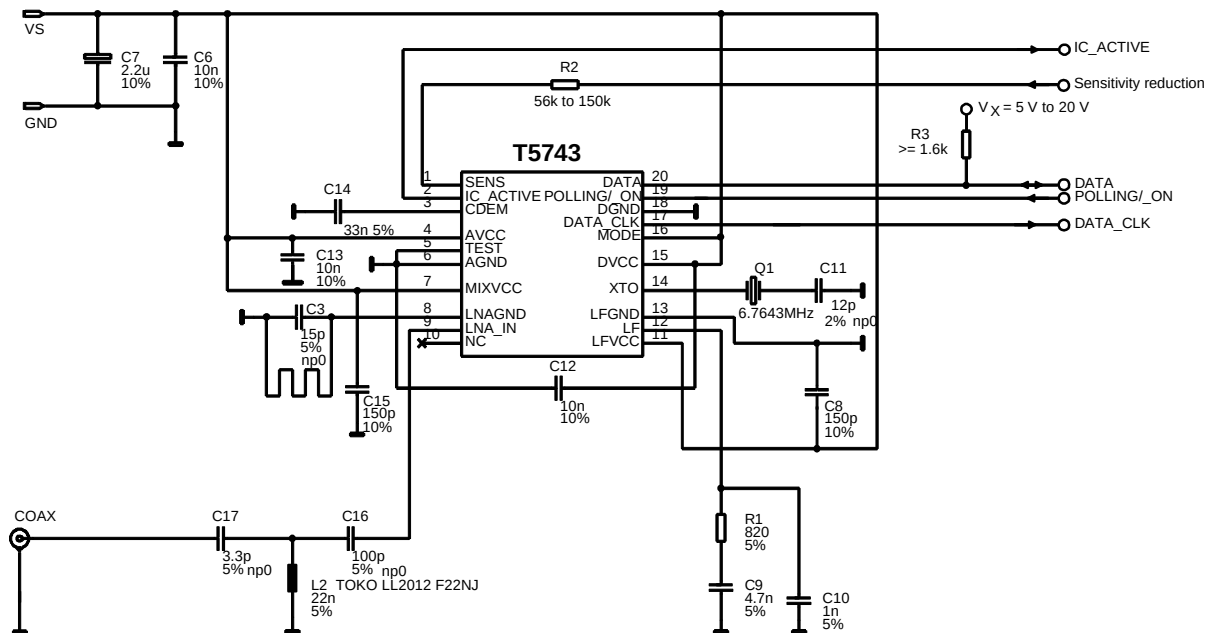
Figure 35. Application Circuit: f_{RF} = 433.92 \text{ MHz} without SAW Filter
